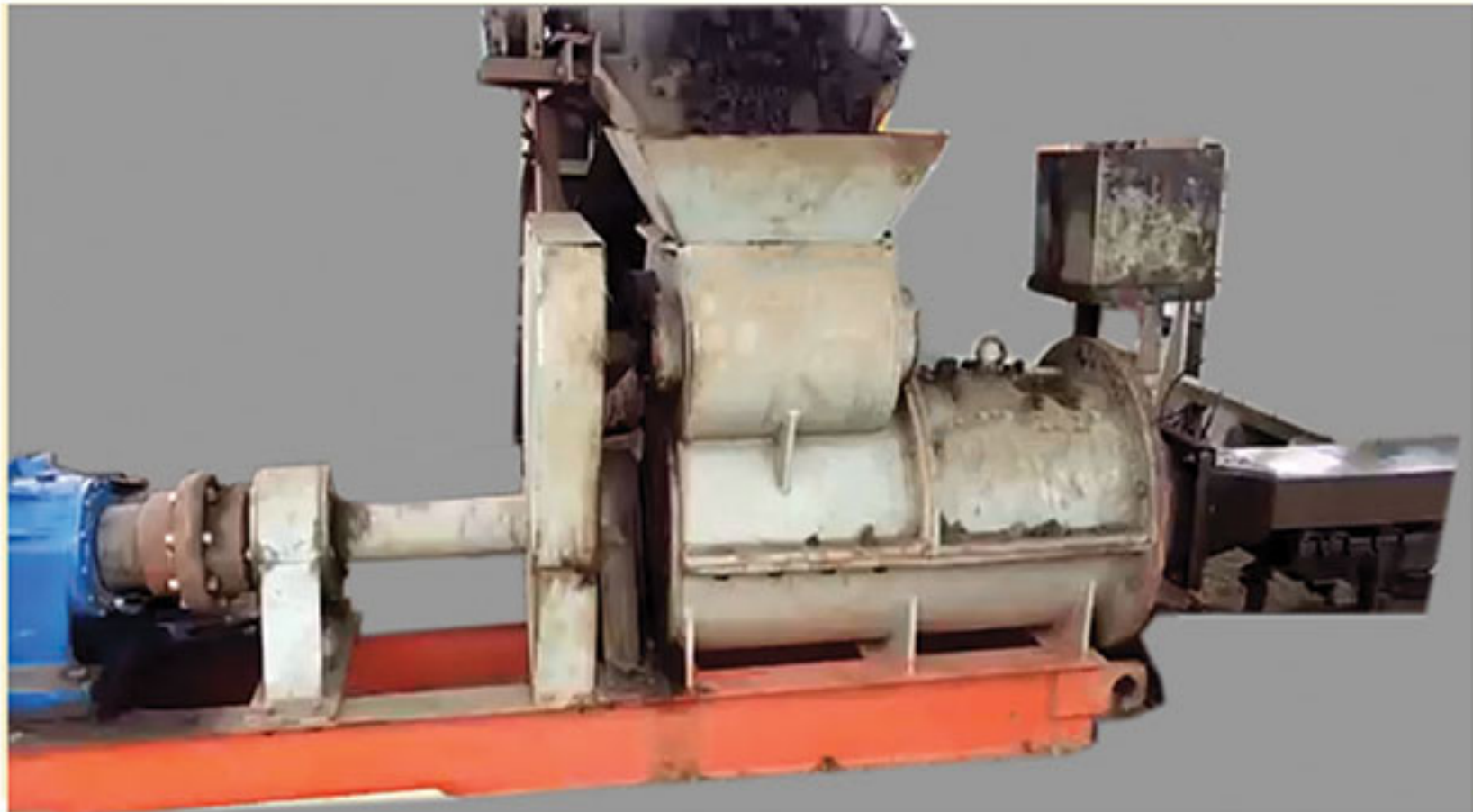
Extruder/ Pugmill
